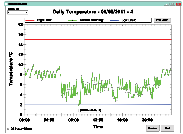
Graph of temperature reading every 5 minutes for each refrigeration unit
